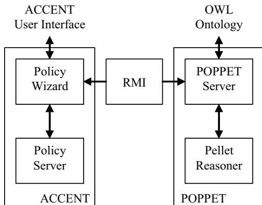
Figure 2. Ontology Integration using POPPET
