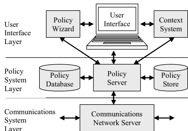
Figure 1. ACCENT Policy System Architecture
