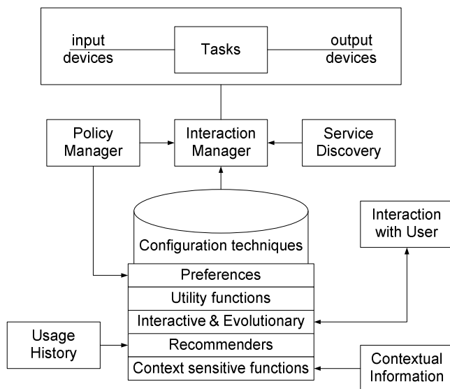
Figure 3. System Architecture
