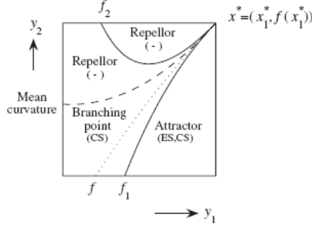
FIG.1: Example of a singular TIP, displaying the coincidence and mutual tangential property of the trade-off f and two invasion boundaries f_1 and f_2 (denoting where s_x(y) = 0 and s_y(x) = 0 respectively) at the tip of the singular TIP (i.e. the top right corner where here y = x = x^* ). The evolutionary behaviour in each region, deduced from the evolutionary properties is also shown. The actual evolutionary behaviour exhibited by the evolutionary singularity x^* is determined by which region the trade-off curve enters, for example, here the evolutionary singularity is a branching point (the singular point is convergence stable (CS) but not evolutionary stable (ES)). The evolutionary outcome of different trade-off shapes can also be considered. If the curvature of the trade-off was such that it entered the TIP below the f_1 line then the singular point would be an evolutionary attractor. If the trade-off entered the TIP above the dashed line (the mean curvature of f_1 and f_2 ) the singular point would be an evolutionary repellor.
