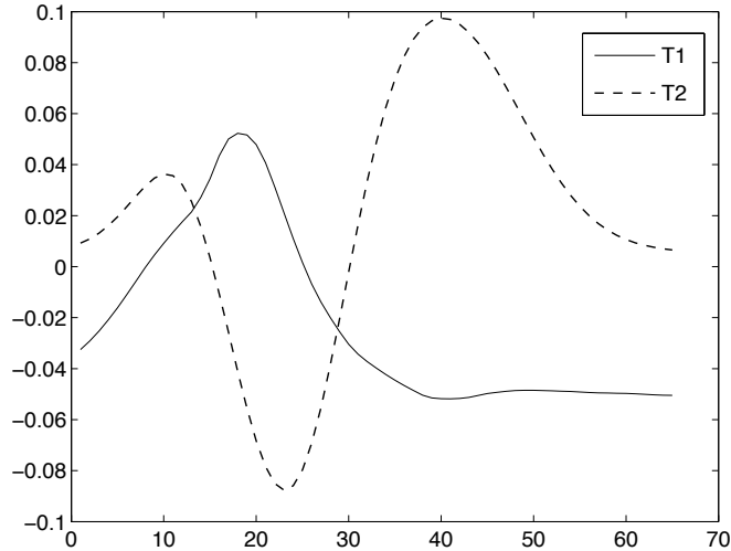
Figure 3. Shapes of the two dissimilar target neuron spikes (T1 and T2) as received at the putative electrode. X axis is in samples at 24 Ksamples/second. Y axis is arbitrary voltage-like units.
