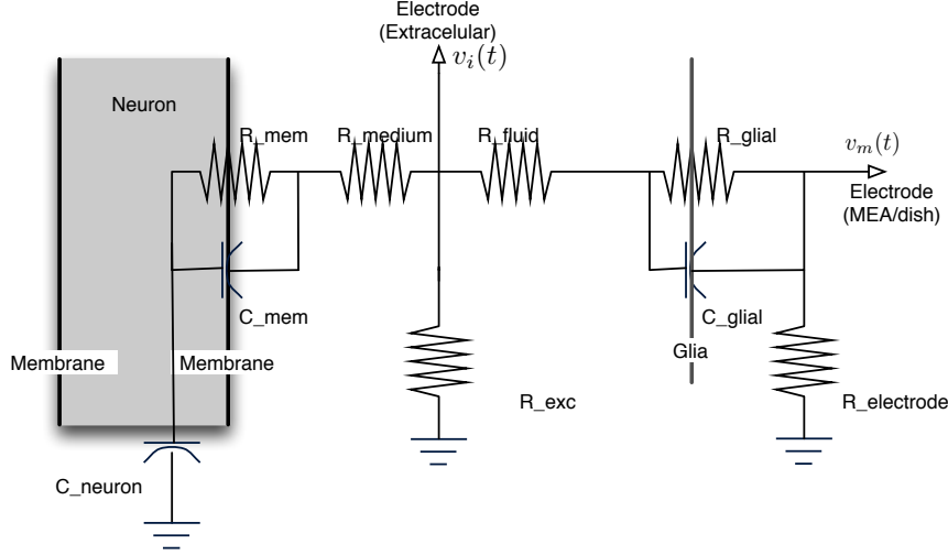
Figure 2. Equivalent circuit description for transfer of charge from a point on a neuron to an electrode for an extracellular and a dish based electrode. The extracellular electrode is assumed to be near the neuron, but the dish electrode is assumed to have a layer of glia between it and the neural culture. There are a number of simplifications in this circuit: distributed resistances and capacitances have been lumped together, for example.
