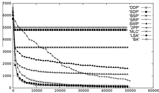
Fig. 2. Average best-so-far objective value over number of evaluations for single heuristic hill-climber on a selected instance (ITC-2007-16). The horizontal axis measures function evaluations, while the vertical axis measures the objective function value.
