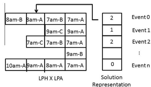
Fig. 1. Representation or encoding of candidate timetable solutions.
