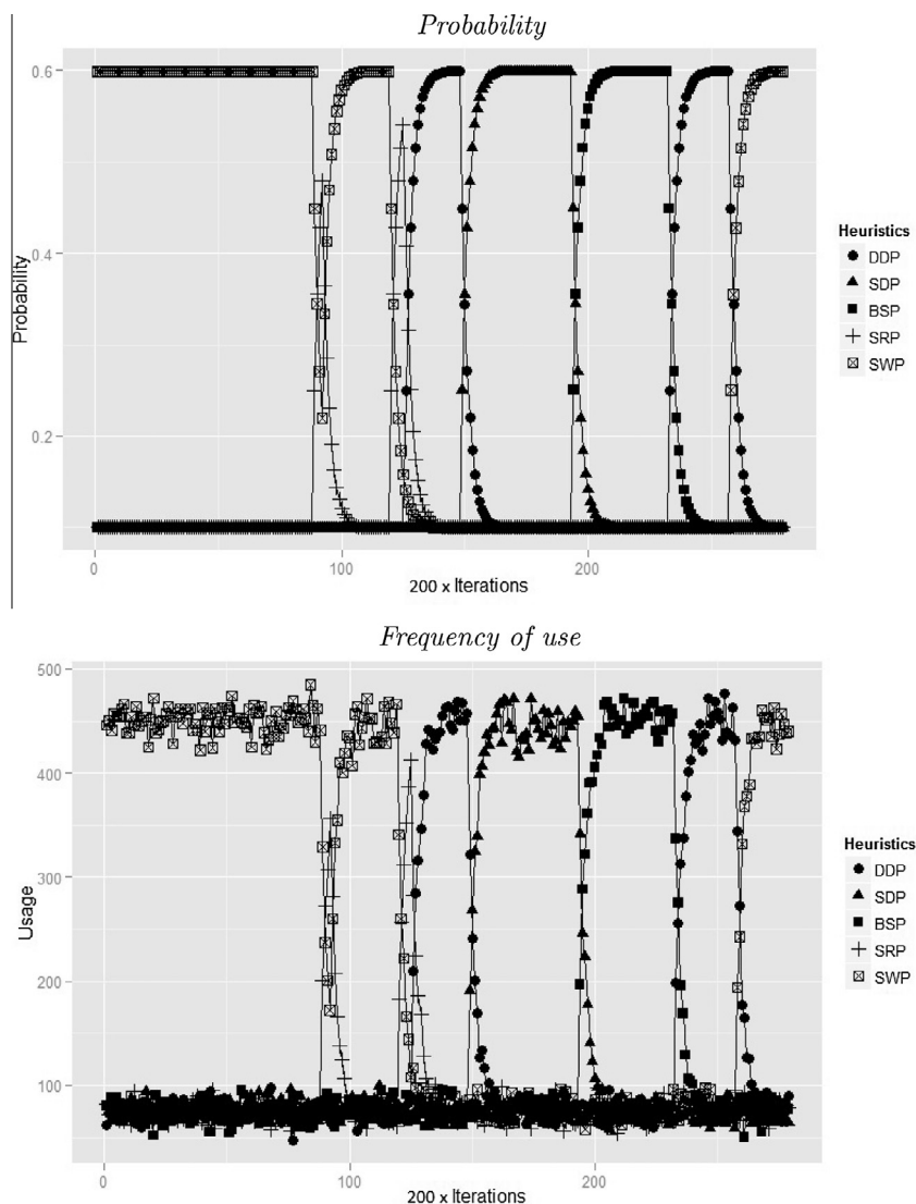
Fig. 3. Instance ITC-2007-9 operator's learned probabilities (top plot) and frequency of use (bottom plot) across a hyper-heuristic run.
