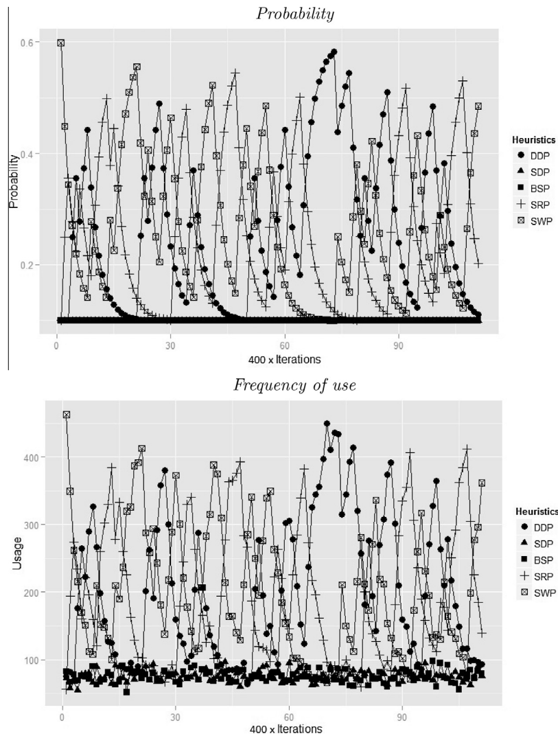
Fig. 4. Instance ITC-2007-13 operator's learned probabilities (top plot) and frequency of use (bottom plot) across a hyper-heuristic run.
