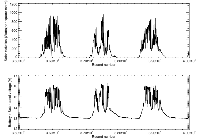
Fig. 5. Three days of data illustrating the correlation between the solar radiation intensity, and the measured solar panel + battery voltage.
