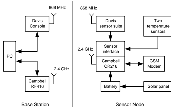
Fig. 2. Components of our first generation prototype node.
