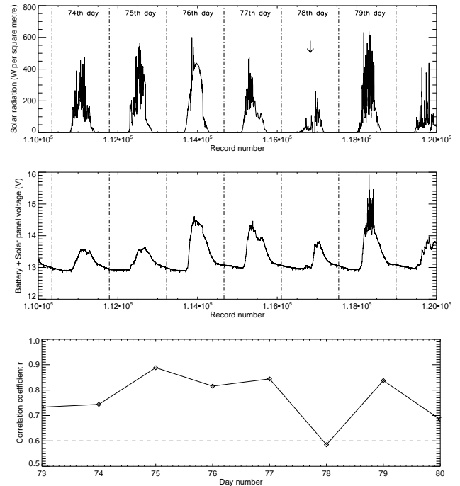
Fig. 8. Solar radiation and solar panel + battery voltage, indicating a forced failure of the solar radiation and detection of the failure.
